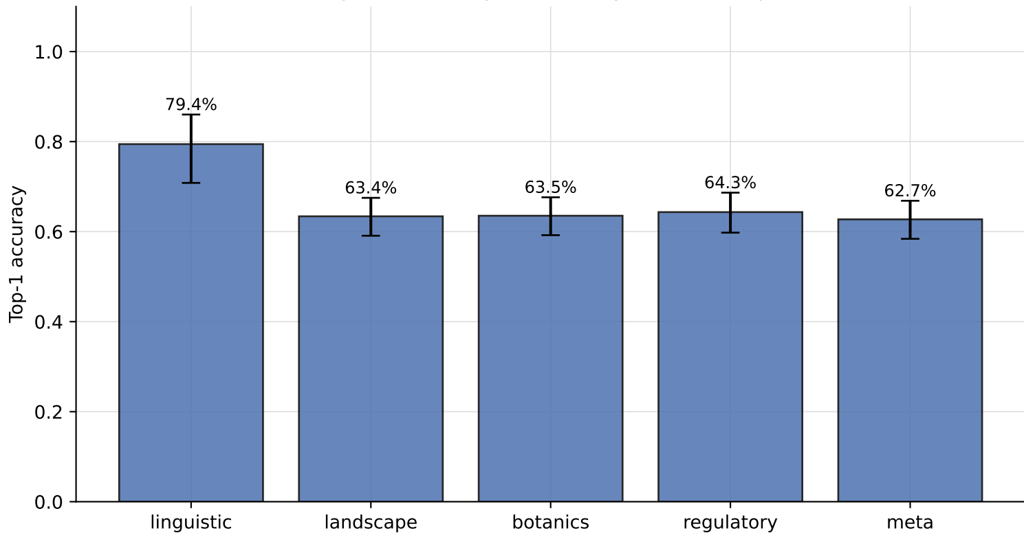
Per-agent initial top-1 accuracy (Hub-and-Spoke)
